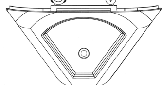
FRONT VIEW - SKIRT
